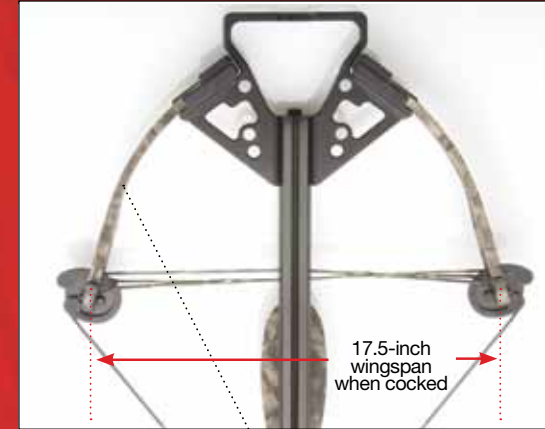
175-pound Defender CLS Bow Assembly
