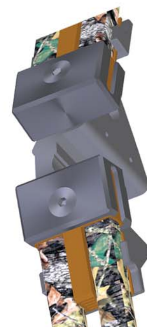
6 Point Riser & Limb Pocket System
