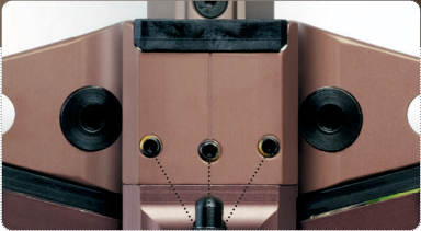
The main assembly bolt's locking setscrew and the foot stirrup's two attachment setscrews are located on the underside of the crossbow's riser (foot stirrup setscrews not applicable to CLS models)
