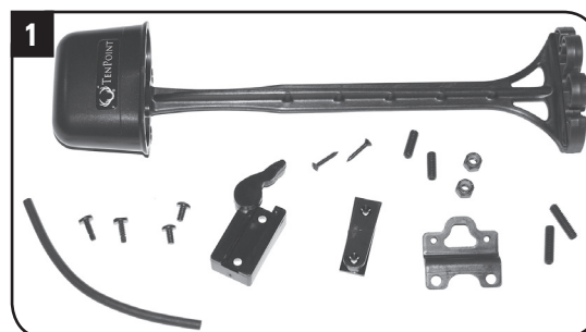
3-Arrow Instant Detach Quiver Mounting Kit
