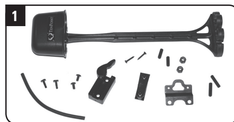
3-Arrow Instant Detach Quiver Mounting Kit
