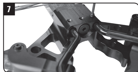
Once the foot stirrup is in place, tighten all three setscrews. See below if mounting the 3-Arrow Instant Detach Quiver.
