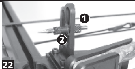
22 1. Elevation lock nut 2. Windage lock nut
