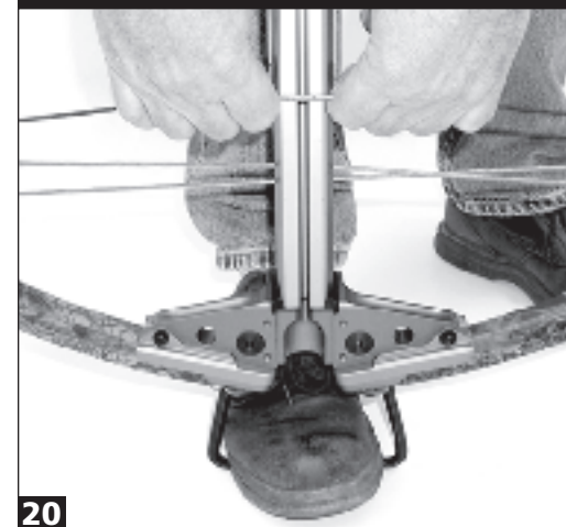
20 If you do not cock your crossbow exactly according to these instructions, chances are you will not group your arrows consistently.
