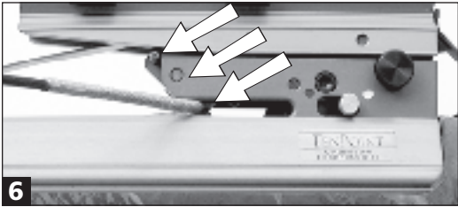
The bowstring will be held by the DFI™ and only appear to be cocked - if you try to load it while the safety is in the SAFE (white dot) position.
