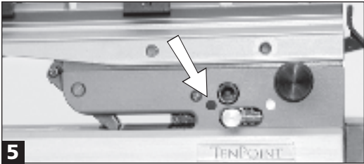
Make sure the trigger's safety is in the FIRE (red dot) position before cocking your crossbow.
