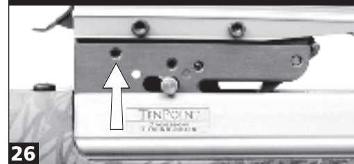
26 The tension-adjustment setscrew.
