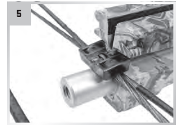
Hold the mini-cross cable saver in position while sliding the bow assembly onto the stock assembly.
