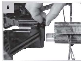
The VIBRA-CUSH goes between the riser and the barrel (on specific models), with the cutout side facing the barrel.
