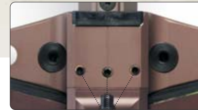
The main assembly bolt's locking setscrew and the foot stirrup's two attachment setscrews are located on the underside of the crossbow's riser (not applicable to the Phantom CLS)
