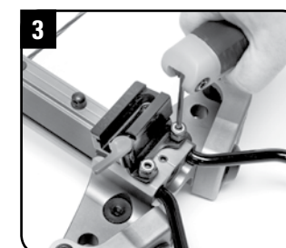
3 Place the quiver bracket assembly over the two setscrew holes and insert 3/4-inch setscrews with Nylock nuts.
