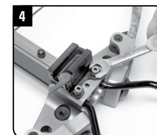
4 Tighten the Nylock nuts with a 7/16-inch open-ended wrench.
