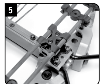
5 Insert the HX Instant Detach Quiver into place and lock in place with the lever.
