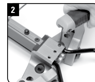
2 Remove 1/4-inch setscrews from the bottom of the riser.
