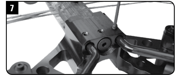
7 Once the foot stirrup is in place, tighten all three setscrews. See below if mounting the HX Instant Detach Quiver.
