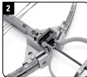
Mount the quiver bracket assembly between the 7/8-inch foot stirrup bolt and the riser.
