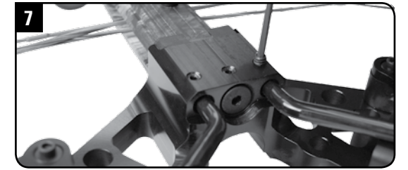
Once the foot stirrup is in place, tighten all three setscrews. See below for mounting the HX Instant Detach Quiver.
